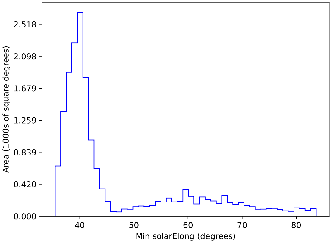
too_elab_r64_d2_giz_v3.4_10yrs WFD all bands: Min solarElong
