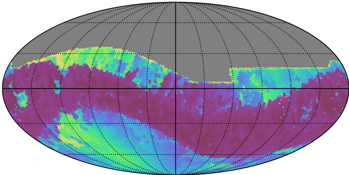
too_elab_r64_d2_giz_v3.4_10yrs All sky z band: Min solarElong
