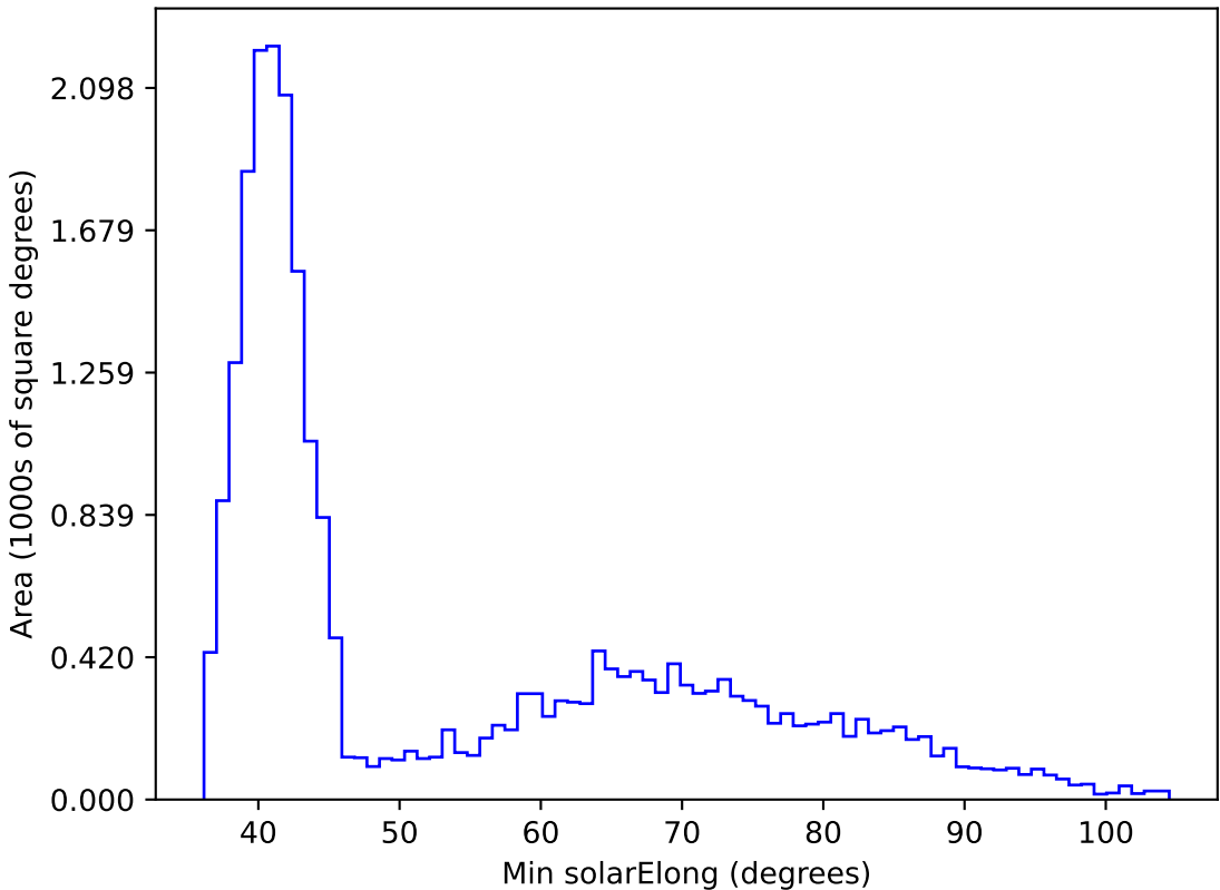
too_elab_r64_d2_giz_v3.4_10yrs All sky z band: Min solarElong
