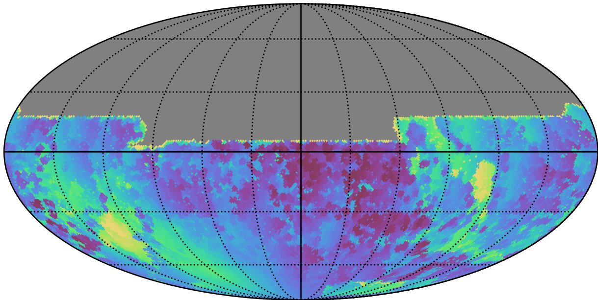
too_elab_r64_d2_giz_v3.4_10yrs All sky y band: Min solarElong
