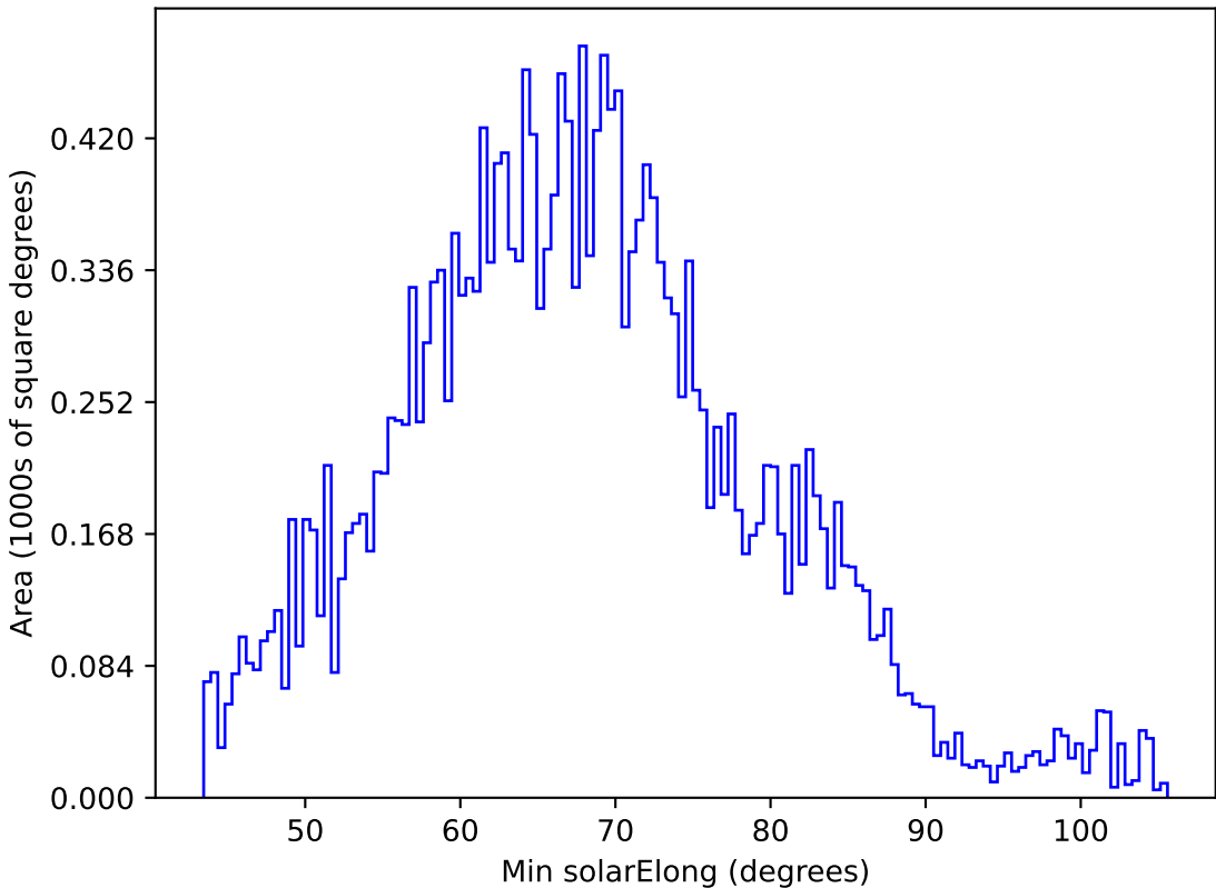
too_elab_r64_d2_giz_v3.4_10yrs All sky y band: Min solarElong
