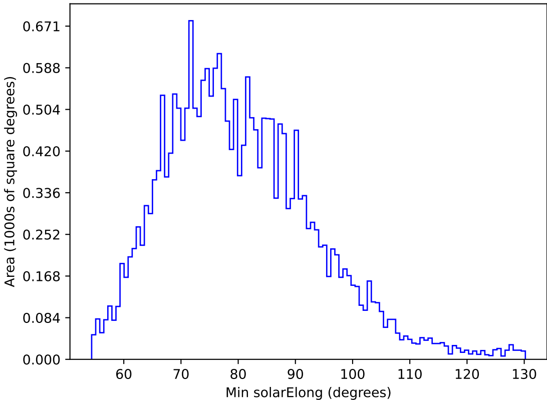
too_elab_r64_d2_giz_v3.4_10yrs All sky u band: Min solarElong
