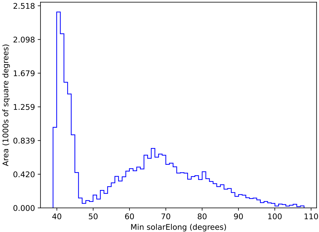
too_elab_r64_d2_giz_v3.4_10yrs All sky r band: Min solarElong
