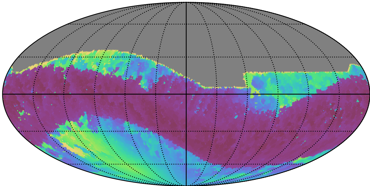
too_elab_r64_d2_giz_v3.4_10yrs All sky i band: Min solarElong
