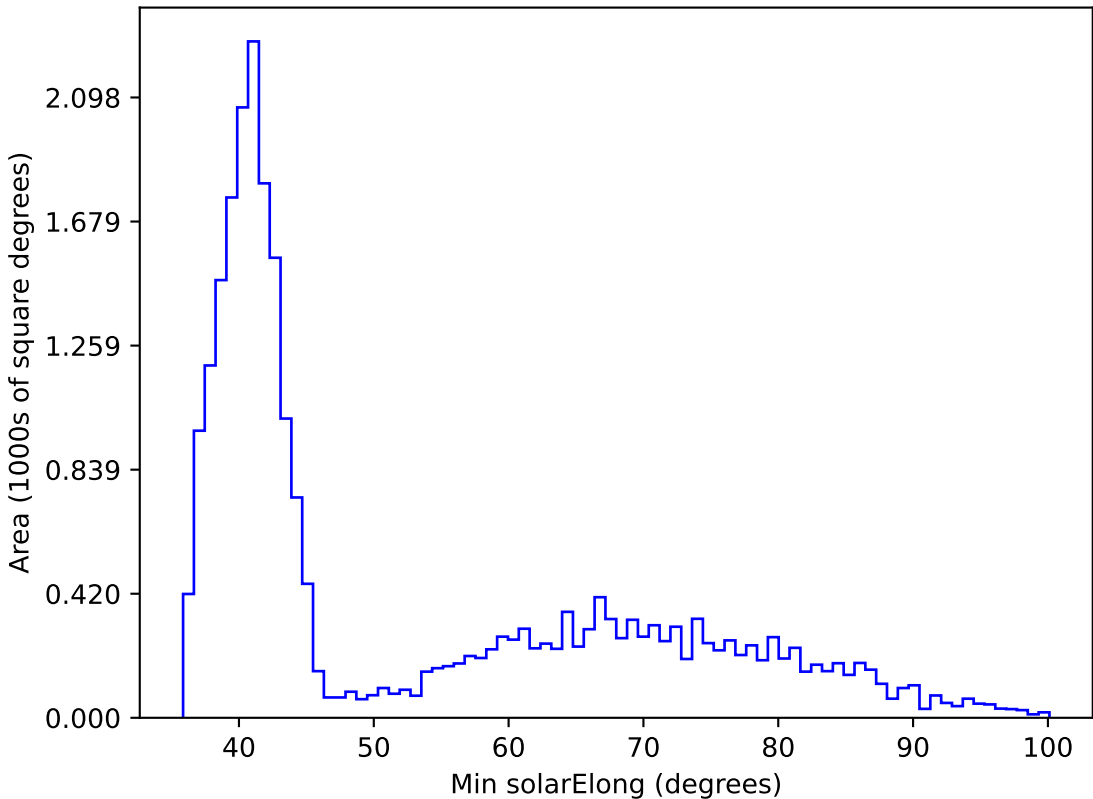
too_elab_r64_d2_giz_v3.4_10yrs All sky i band: Min solarElong
