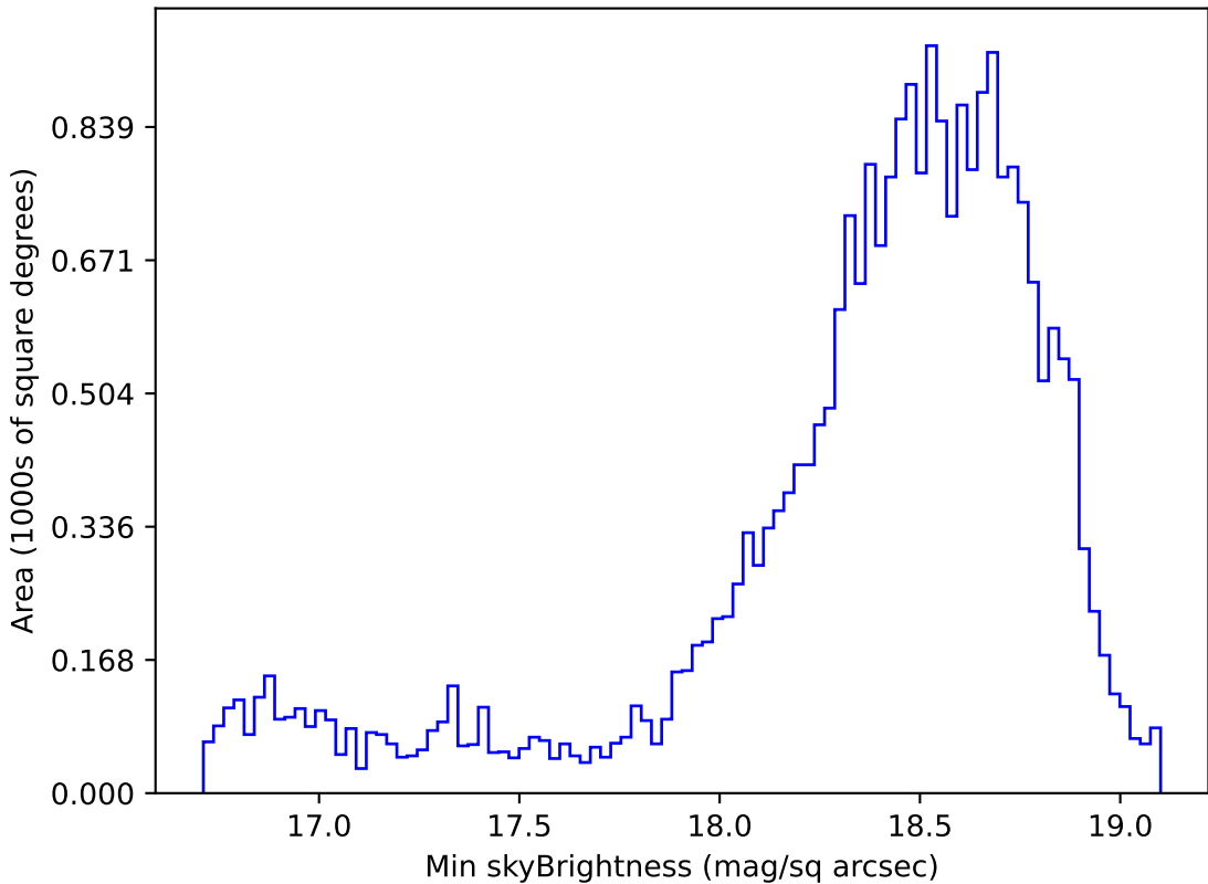
too_elab_r64_d2_giz_v3.4_10yrs Yr 1 z band: Min skyBrightness
