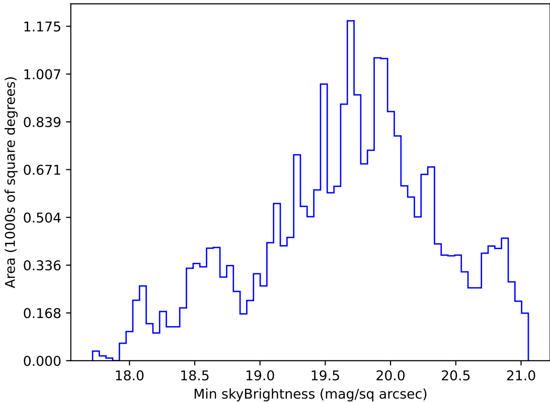
too_elab_r64_d2_giz_v3.4_10yrs Yr 1 r band: Min skyBrightness
