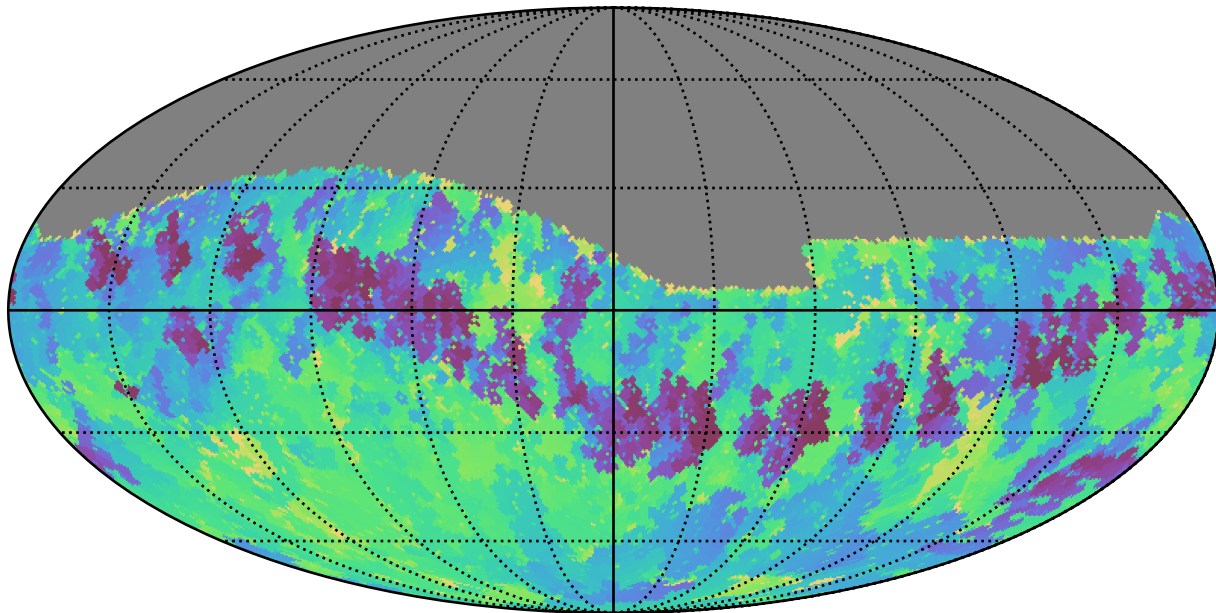
too_elab_r64_d2_giz_v3.4_10yrs Yr 1 i band: Min skyBrightness
