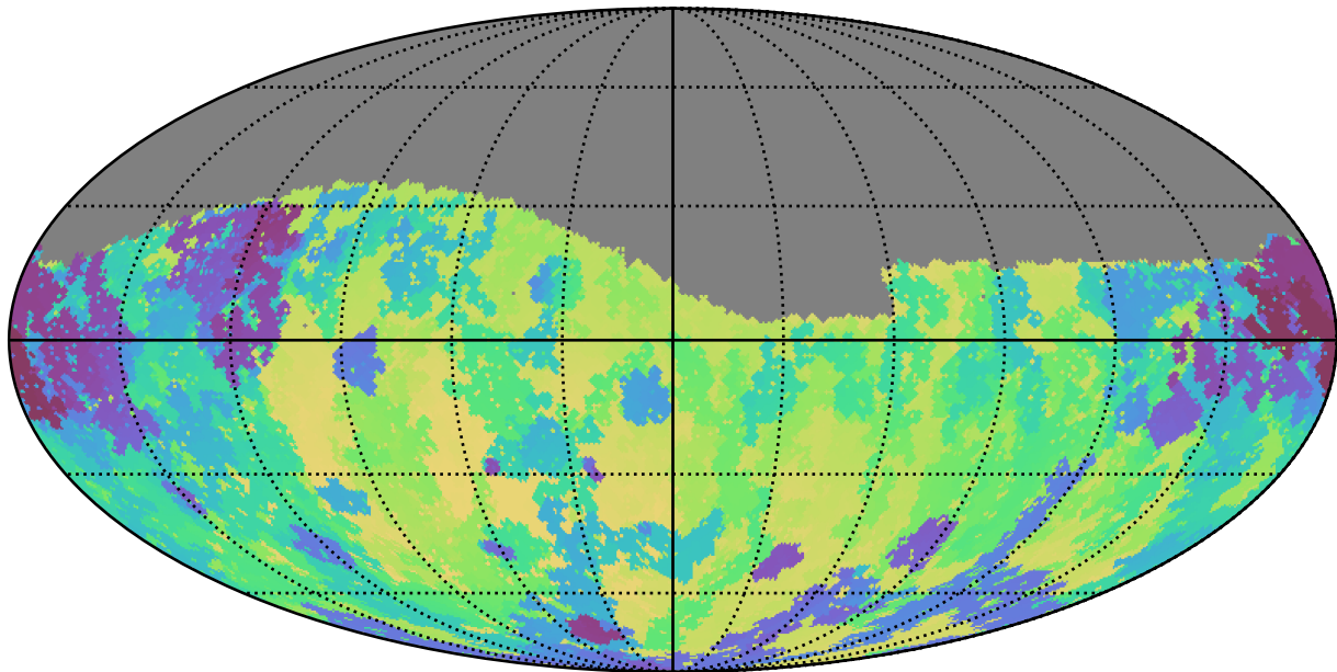
too_elab_r64_d2_giz_v3.4_10yrs Yr 1 g band: Min skyBrightness
