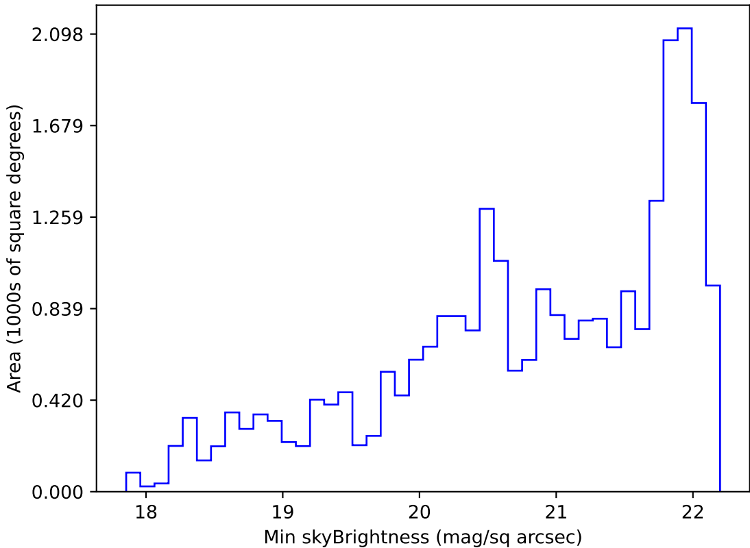
too_elab_r64_d2_giz_v3.4_10yrs Yr 1 g band: Min skyBrightness
