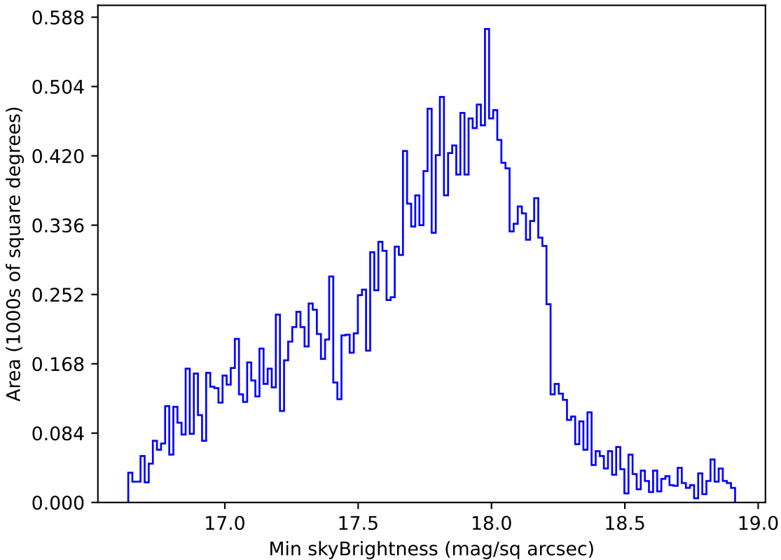
too_elab_r64_d2_giz_v3.4_10yrs Yr 1 all bands: Min skyBrightness
