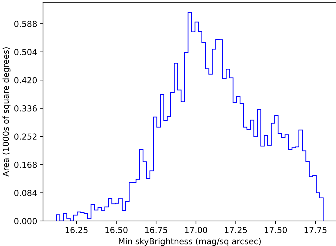
too_elab_r64_d2_giz_v3.4_10yrs WFD y band: Min skyBrightness
