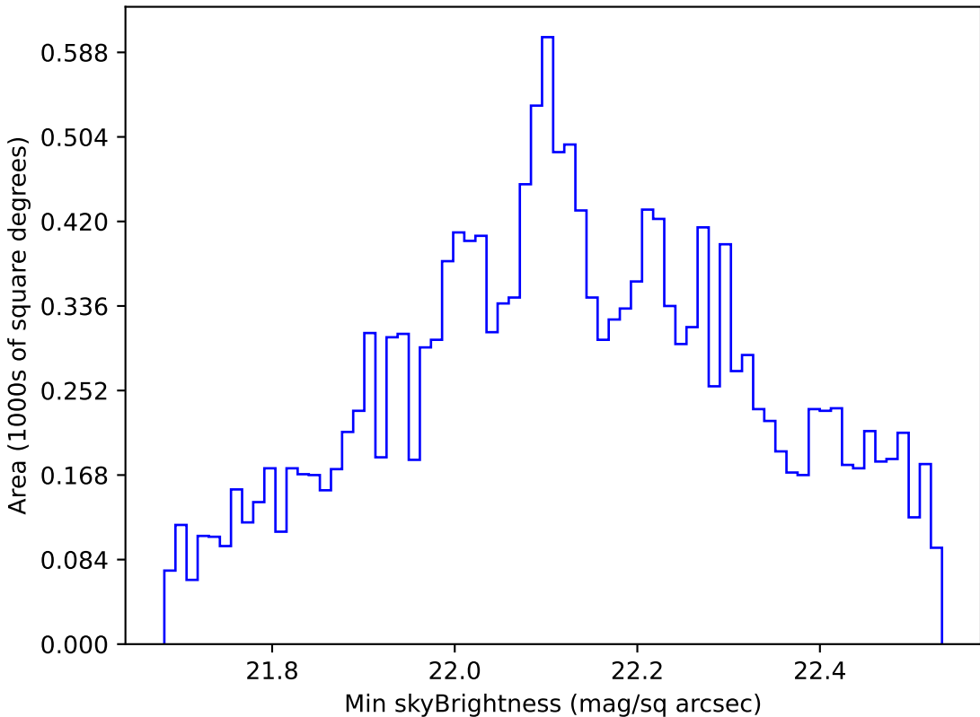
too_elab_r64_d2_giz_v3.4_10yrs WFD u band: Min skyBrightness
