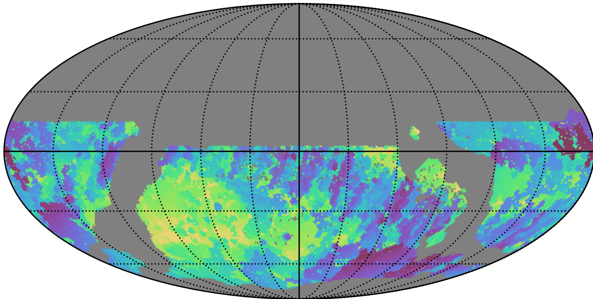
too_elab_r64_d2_giz_v3.4_10yrs WFD r band: Min skyBrightness
