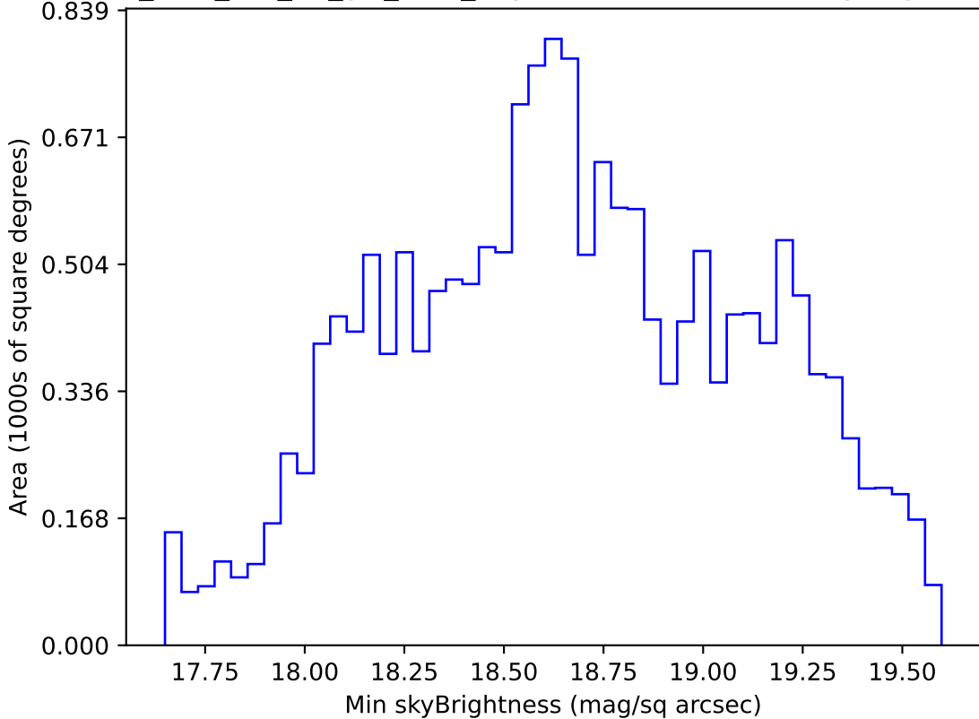
too_elab_r64_d2_giz_v3.4_10yrs WFD r band: Min skyBrightness
