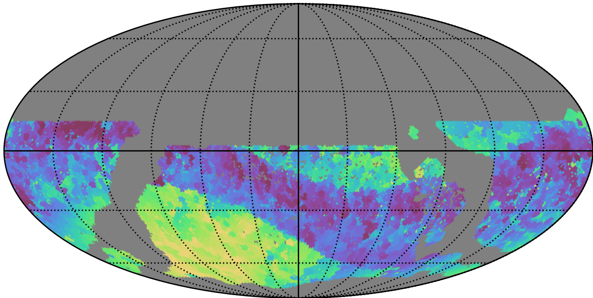
too_elab_r64_d2_giz_v3.4_10yrs WFD i band: Min skyBrightness
