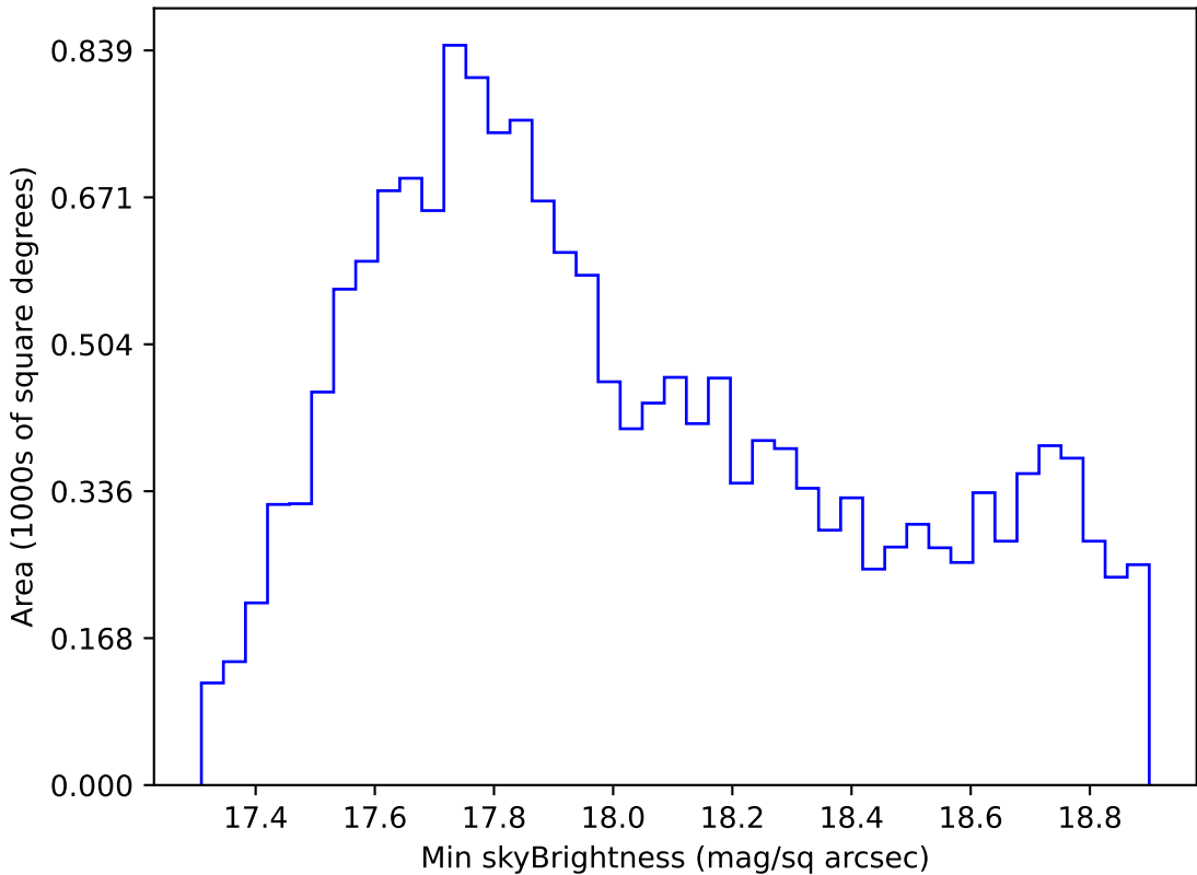
too_elab_r64_d2_giz_v3.4_10yrs WFD i band: Min skyBrightness
