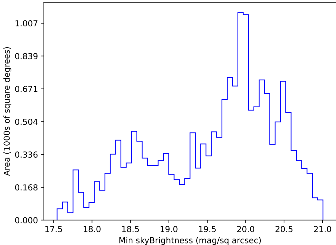
too_elab_r64_d2_giz_v3.4_10yrs WFD g band: Min skyBrightness
