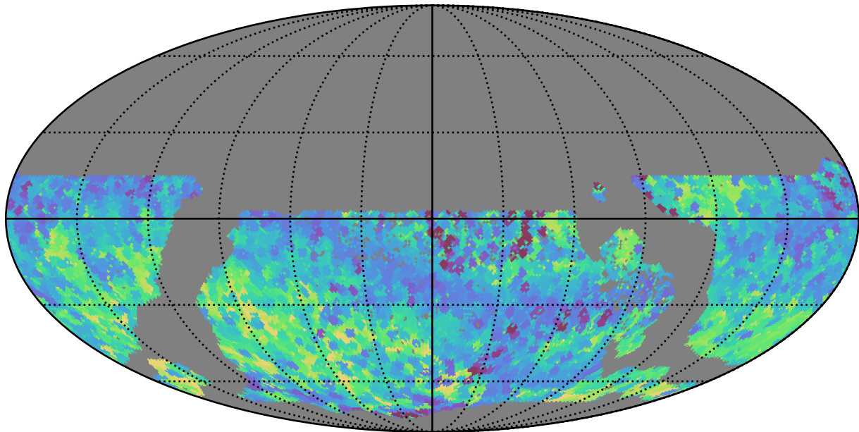
too_elab_r64_d2_giz_v3.4_10yrs WFD all bands: Min skyBrightness
