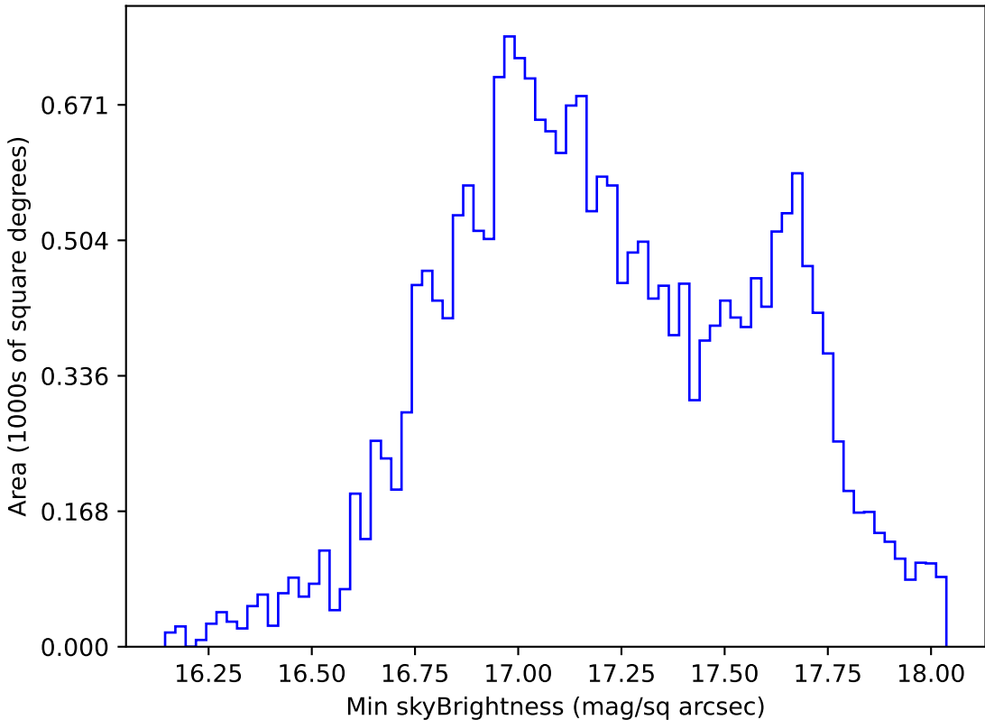
too_elab_r64_d2_giz_v3.4_10yrs All sky y band: Min skyBrightness
