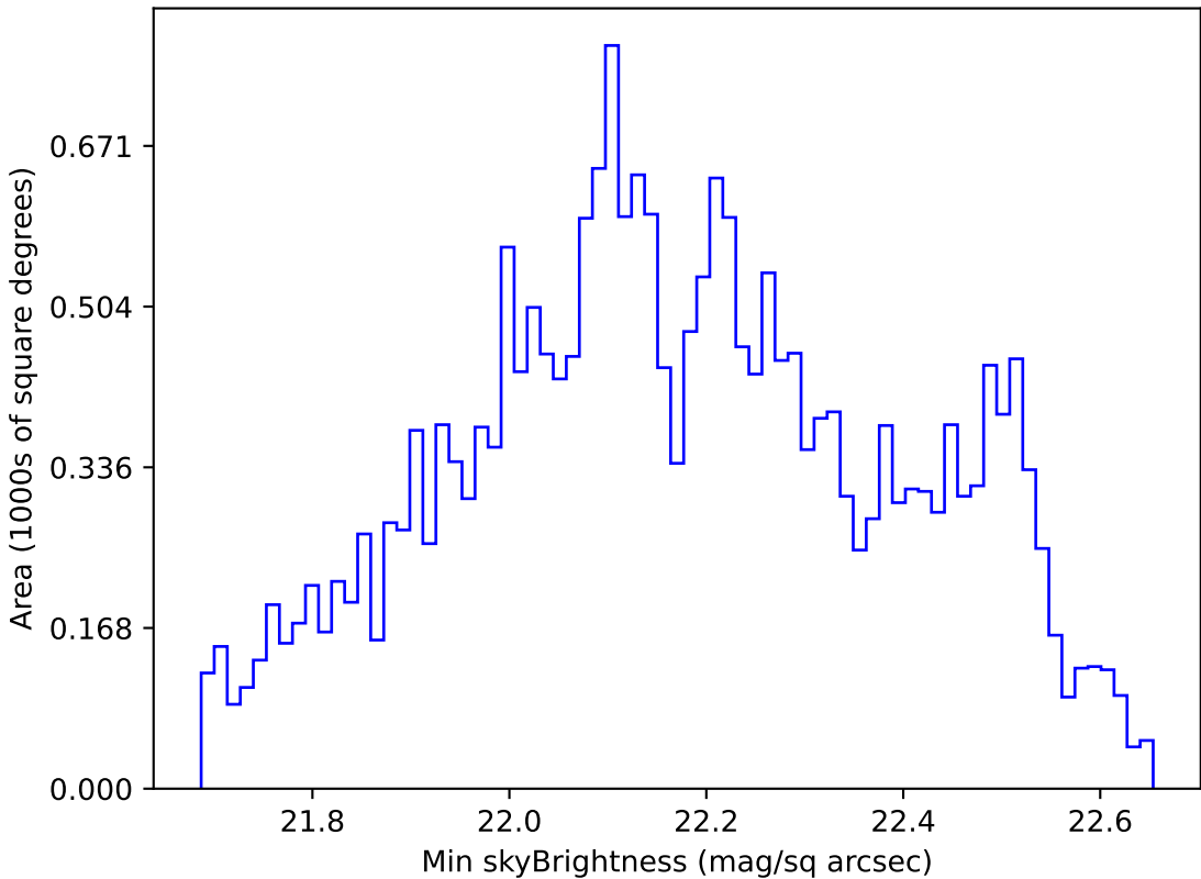
too_elab_r64_d2_giz_v3.4_10yrs All sky u band: Min skyBrightness
