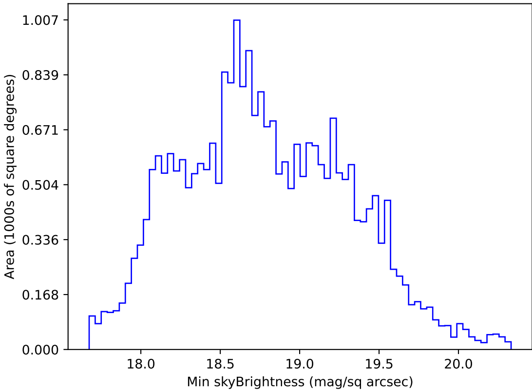
too_elab_r64_d2_giz_v3.4_10yrs All sky r band: Min skyBrightness
