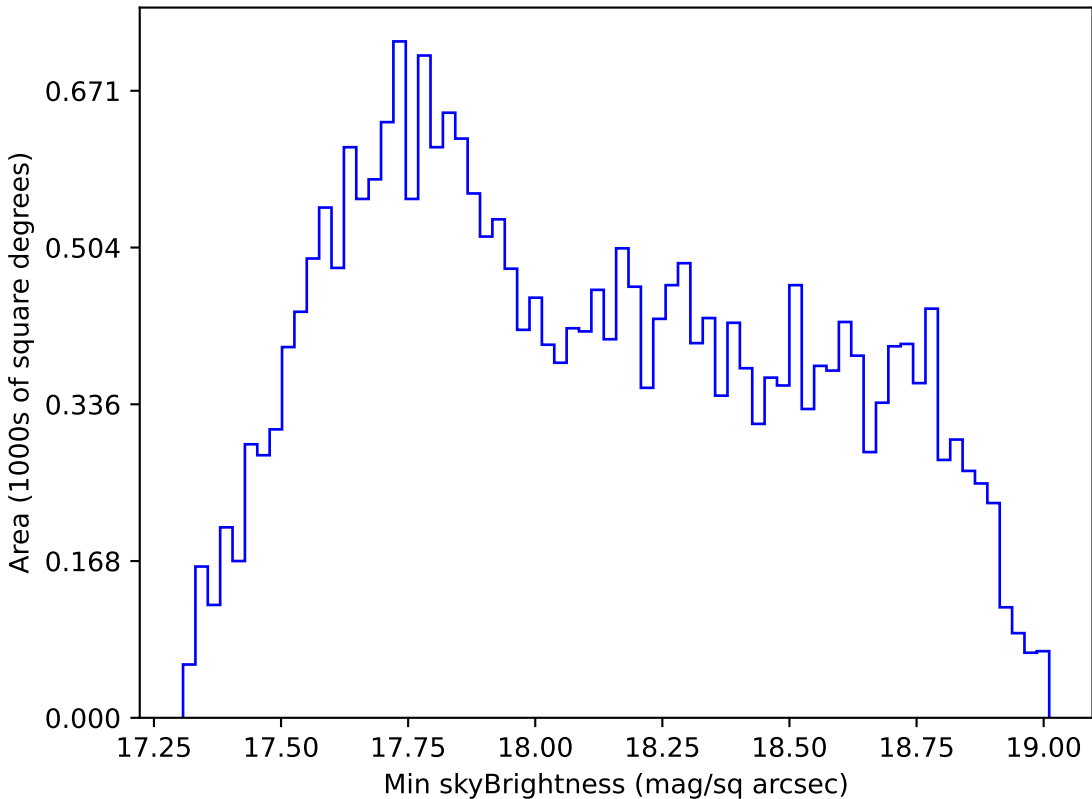
too_elab_r64_d2_giz_v3.4_10yrs All sky i band: Min skyBrightness
