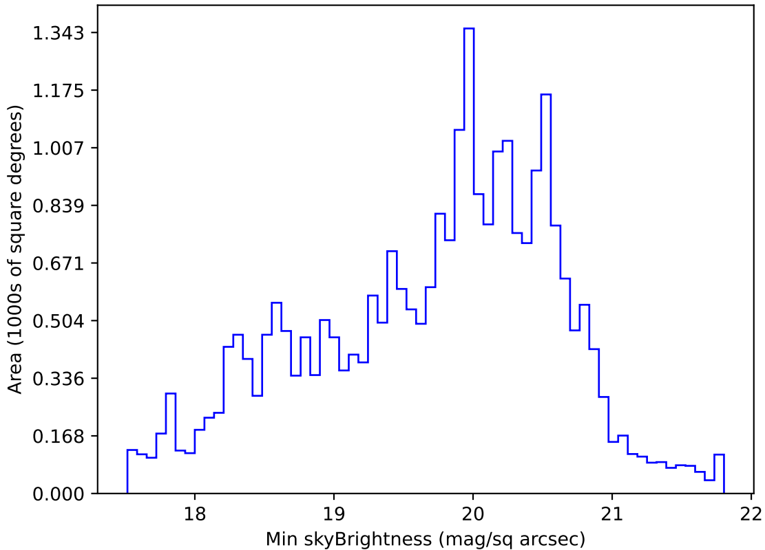
too_elab_r64_d2_giz_v3.4_10yrs All sky g band: Min skyBrightness
