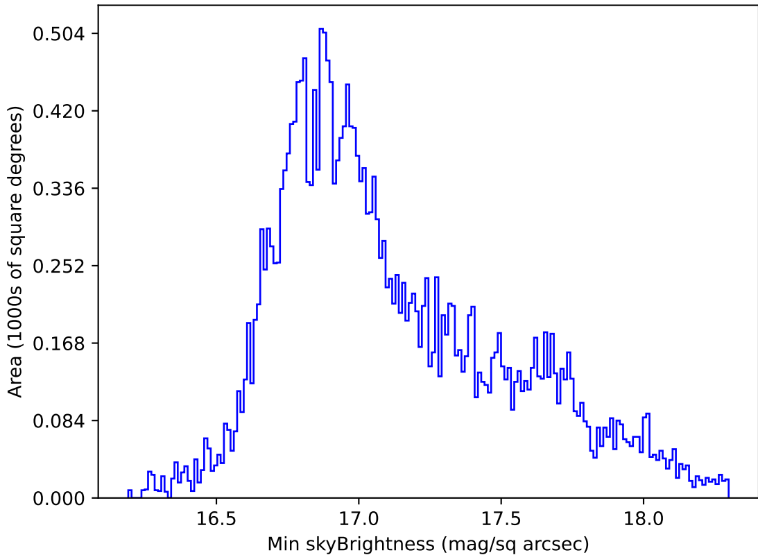
too_elab_r64_d2_giz_v3.4_10yrs All sky all bands: Min skyBrightness
