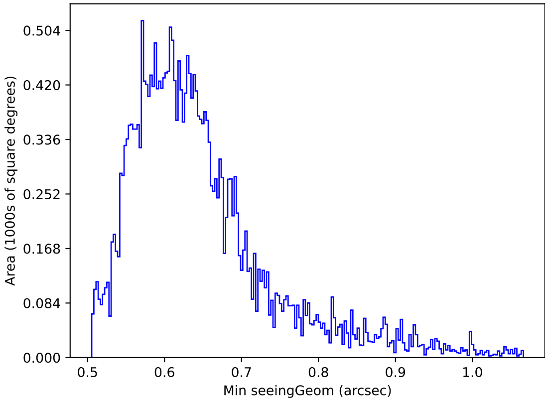
too_elab_r64_d2_giz_v3.4_10yrs Yr 1 z band: Min seeingGeom
