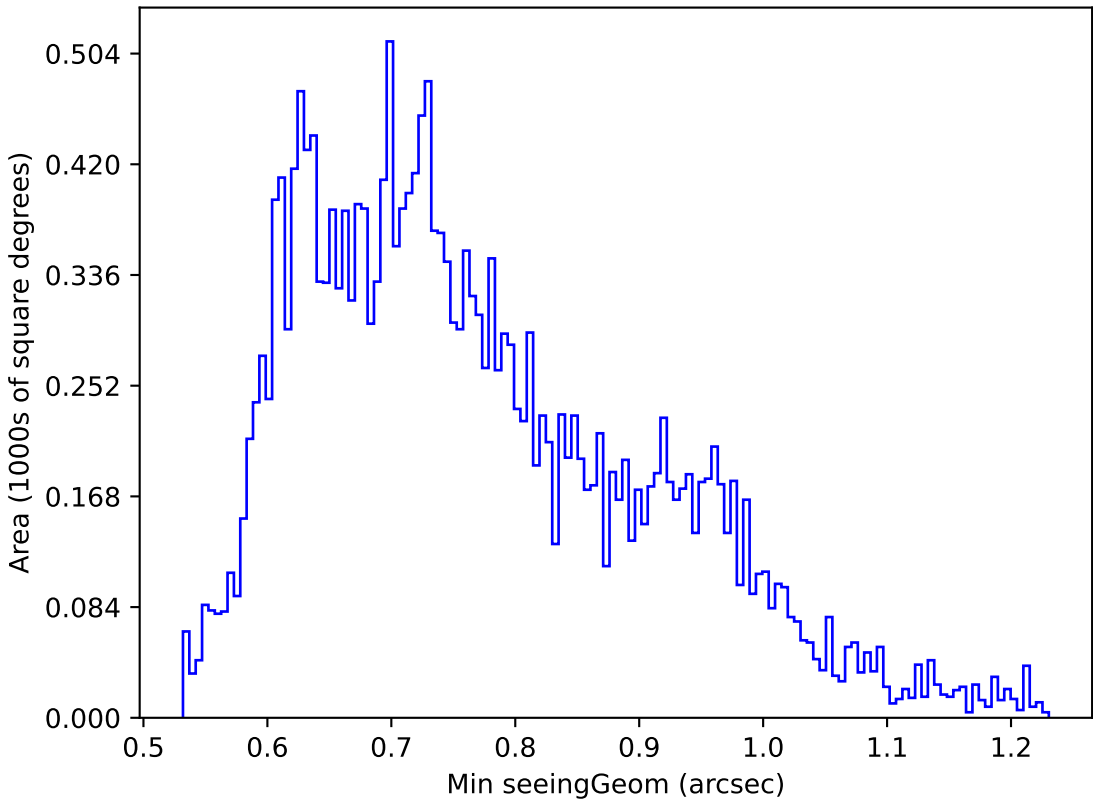
too_elab_r64_d2_giz_v3.4_10yrs Yr 1 u band: Min seeingGeom
