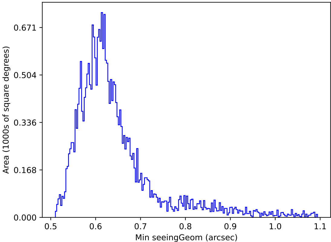
too_elab_r64_d2_giz_v3.4_10yrs Yr 1 r band: Min seeingGeom
