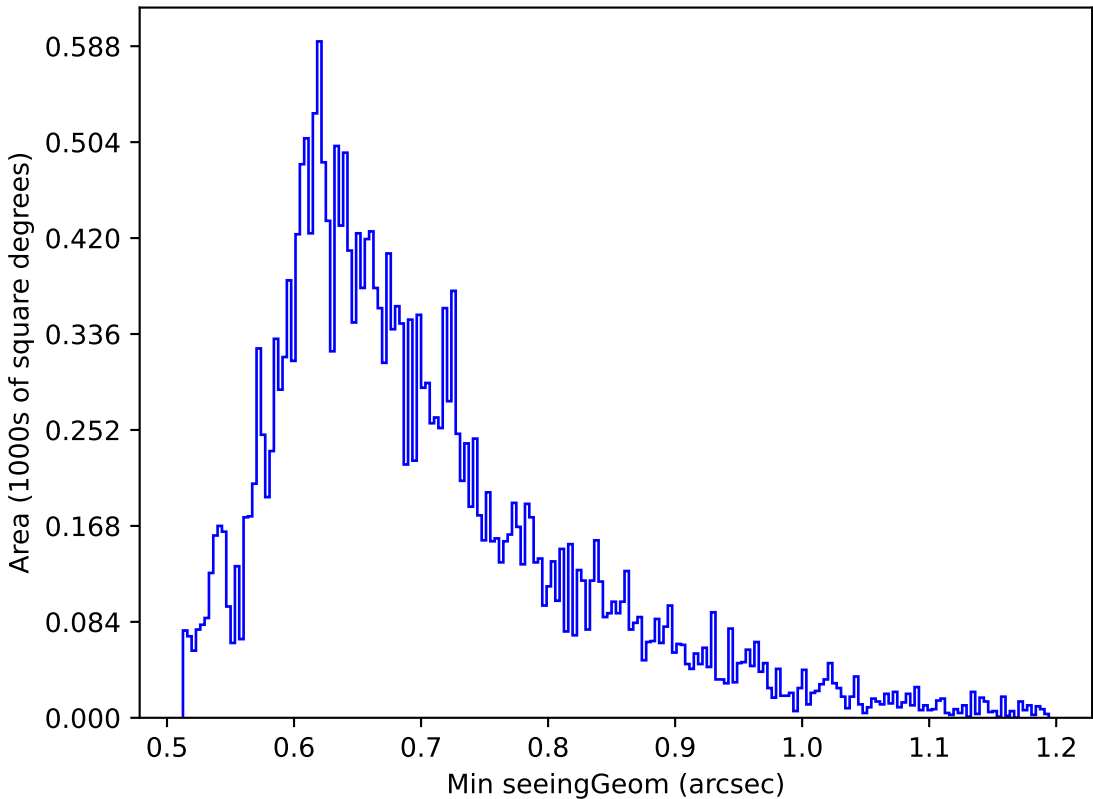
too_elab_r64_d2_giz_v3.4_10yrs Yr 1 g band: Min seeingGeom
