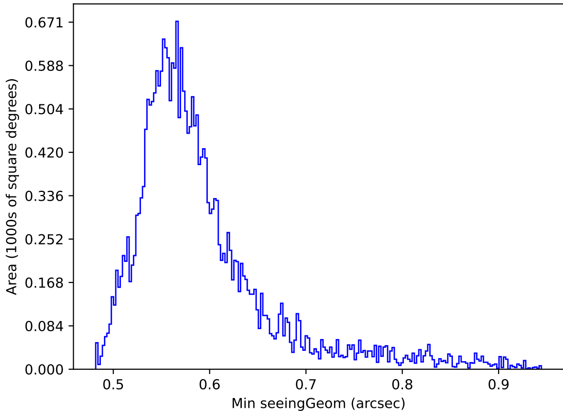
too_elab_r64_d2_giz_v3.4_10yrs Yr 1 all bands: Min seeingGeom
