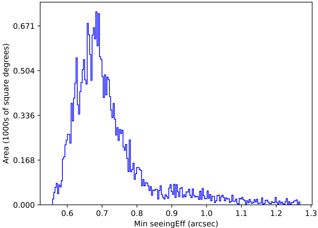
too_elab_r64_d2_giz_v3.4_10yrs Yr 1 r band: Min seeingEff
