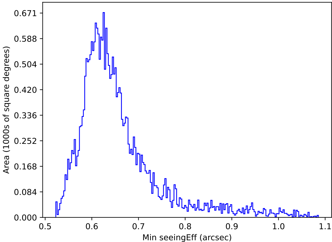
too_elab_r64_d2_giz_v3.4_10yrs Yr 1 all bands: Min seeingEff
