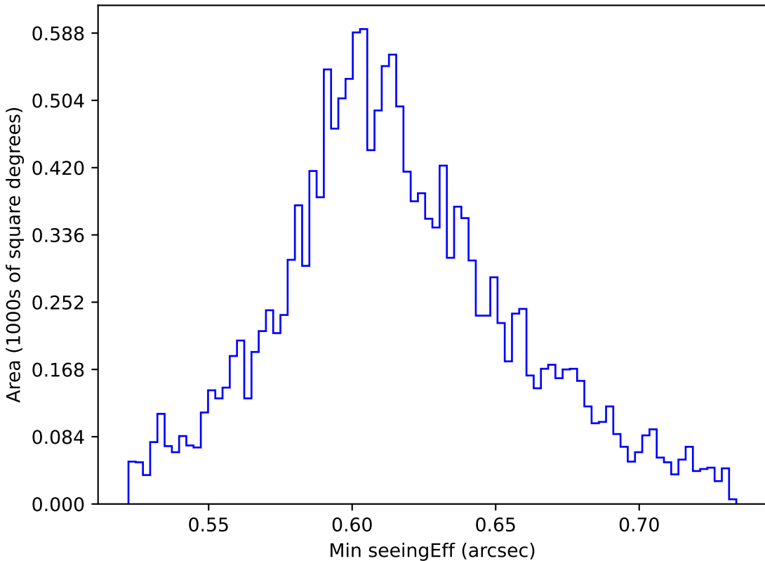
too_elab_r64_d2_giz_v3.4_10yrs WFD z band: Min seeingEff
