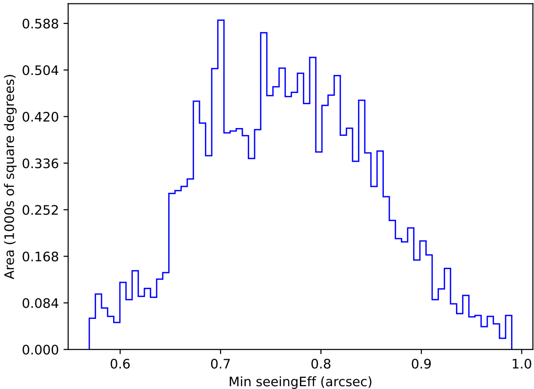
too_elab_r64_d2_giz_v3.4_10yrs WFD u band: Min seeingEff
