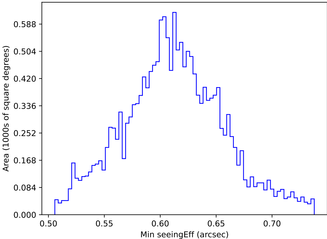
too_elab_r64_d2_giz_v3.4_10yrs WFD r band: Min seeingEff
