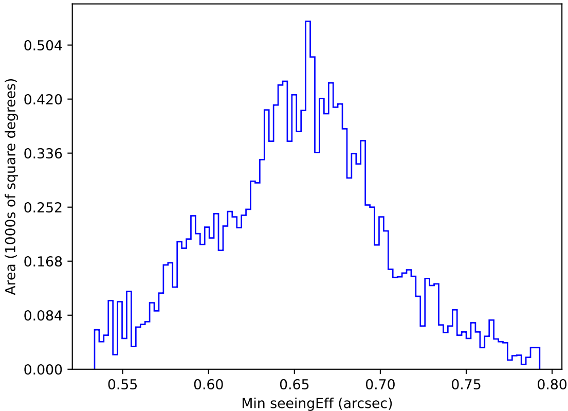
too_elab_r64_d2_giz_v3.4_10yrs WFD g band: Min seeingEff
