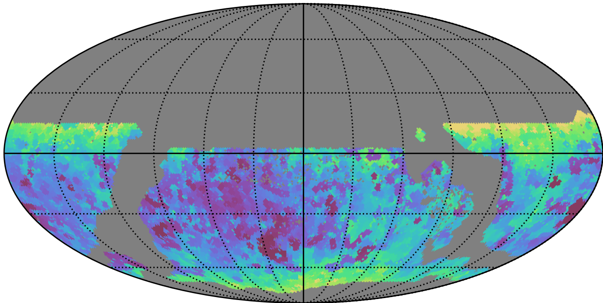
too_elab_r64_d2_giz_v3.4_10yrs WFD all bands: Min seeingEff
