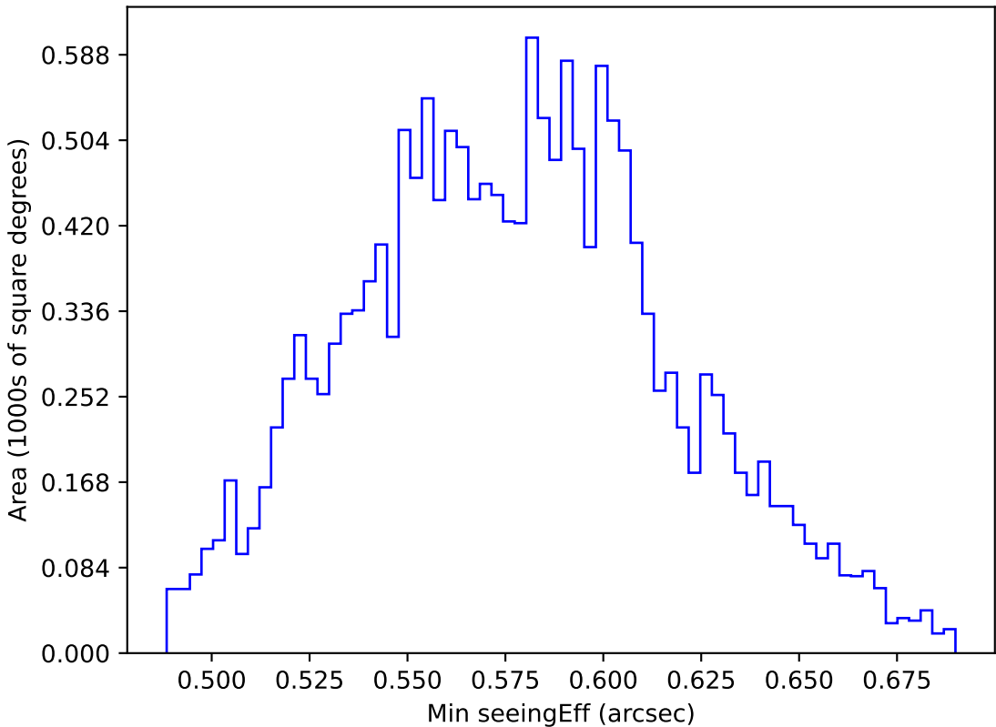
too_elab_r64_d2_giz_v3.4_10yrs WFD all bands: Min seeingEff
