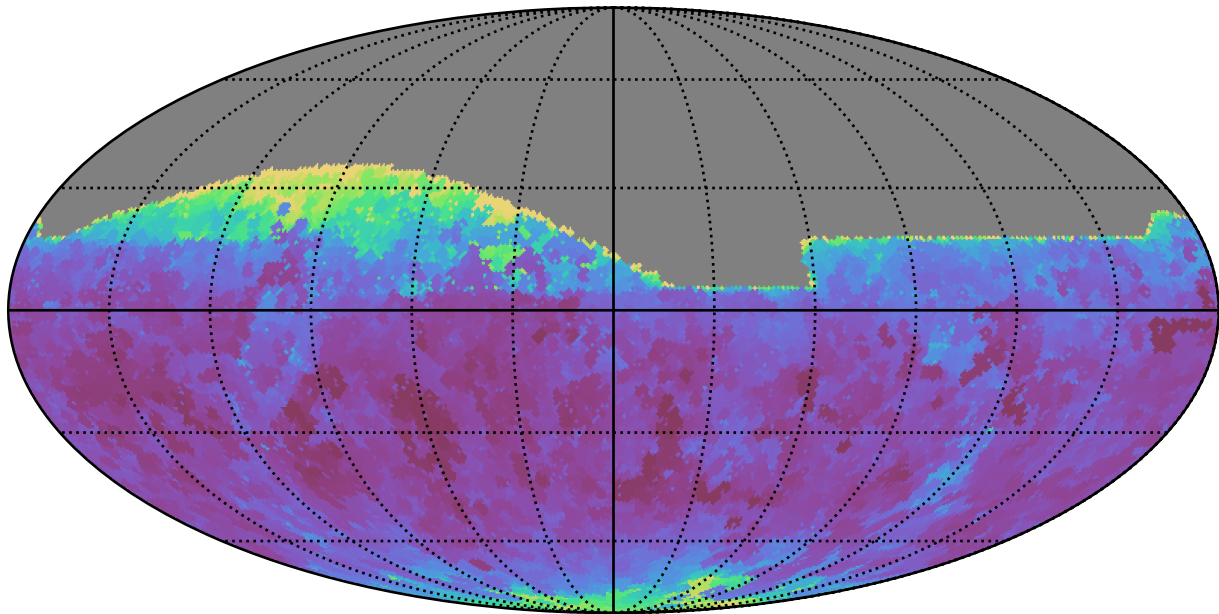
too_elab_r64_d2_giz_v3.4_10yrs All sky z band: Min seeingEff
