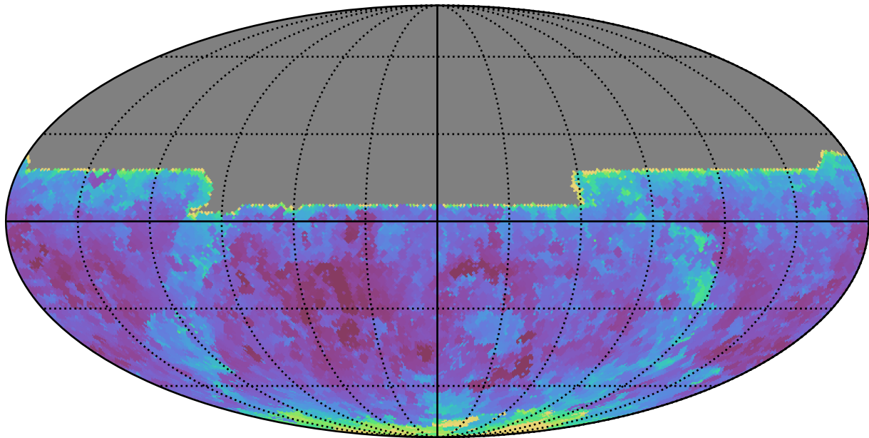
too_elab_r64_d2_giz_v3.4_10yrs All sky y band: Min seeingEff
