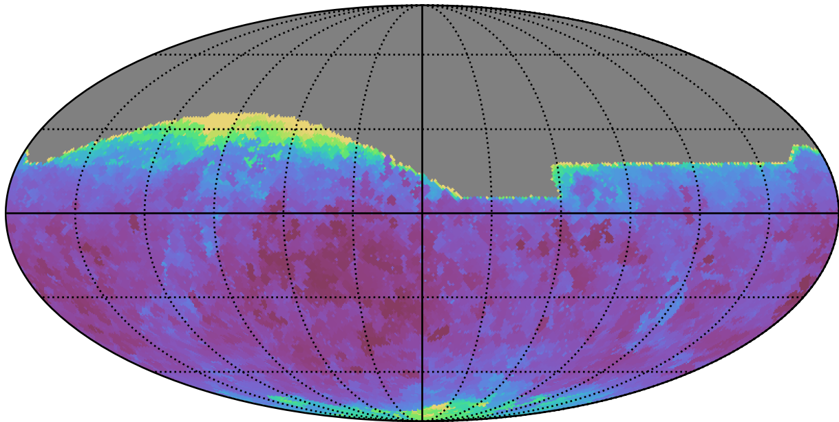
too_elab_r64_d2_giz_v3.4_10yrs All sky r band: Min seeingEff
