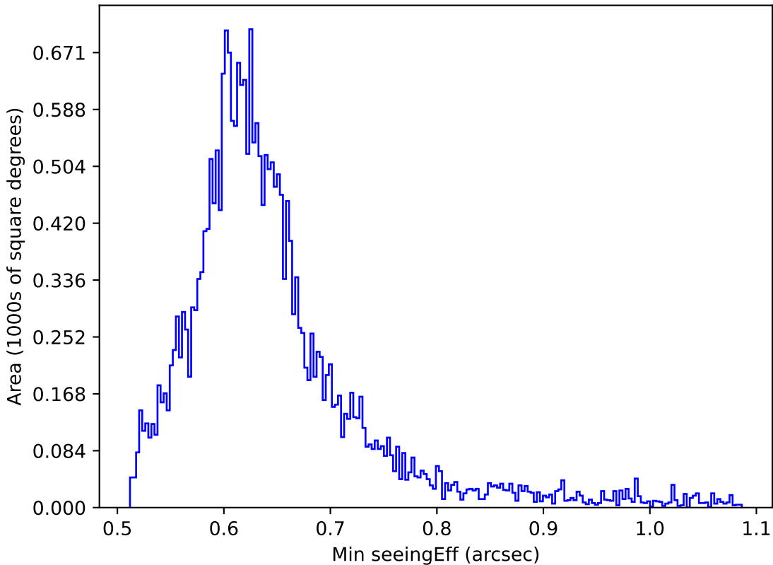
too_elab_r64_d2_giz_v3.4_10yrs All sky r band: Min seeingEff
