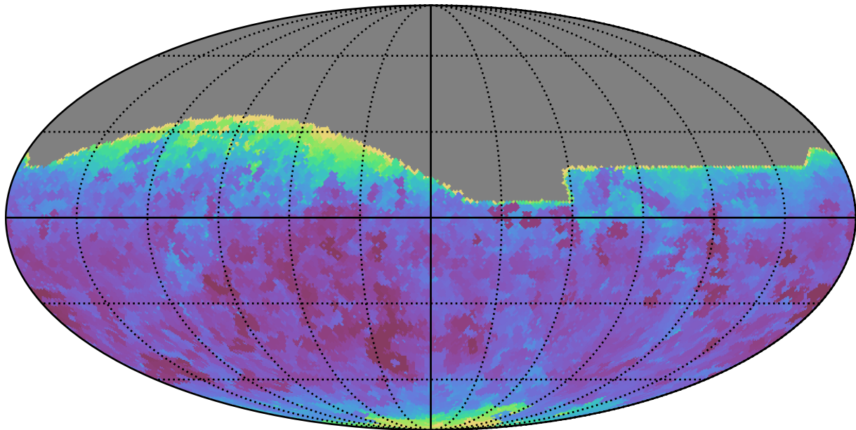
too_elab_r64_d2_giz_v3.4_10yrs All sky i band: Min seeingEff
