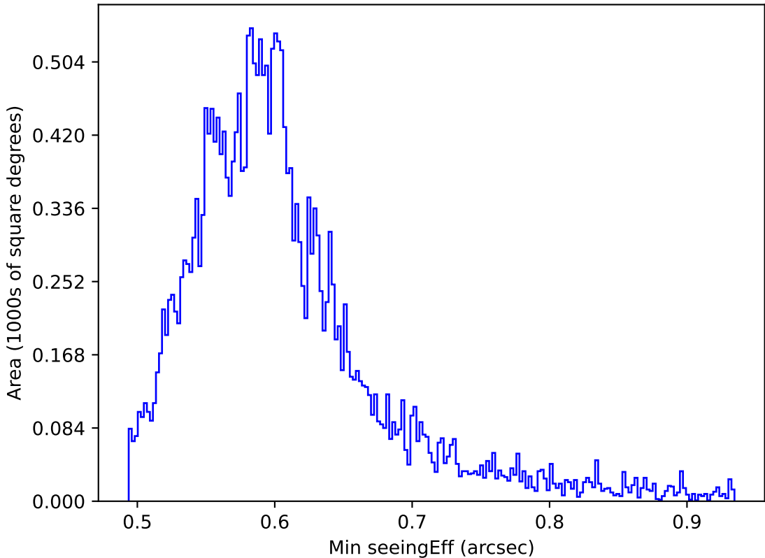
too_elab_r64_d2_giz_v3.4_10yrs All sky all bands: Min seeingEff
