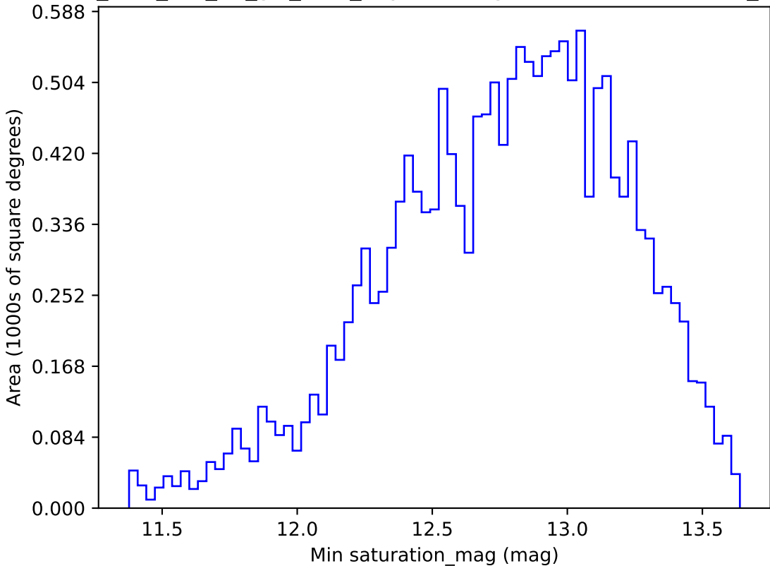
too_elab_r64_d2_giz_v3.4_10yrs WFD g band: Min saturation_mag
