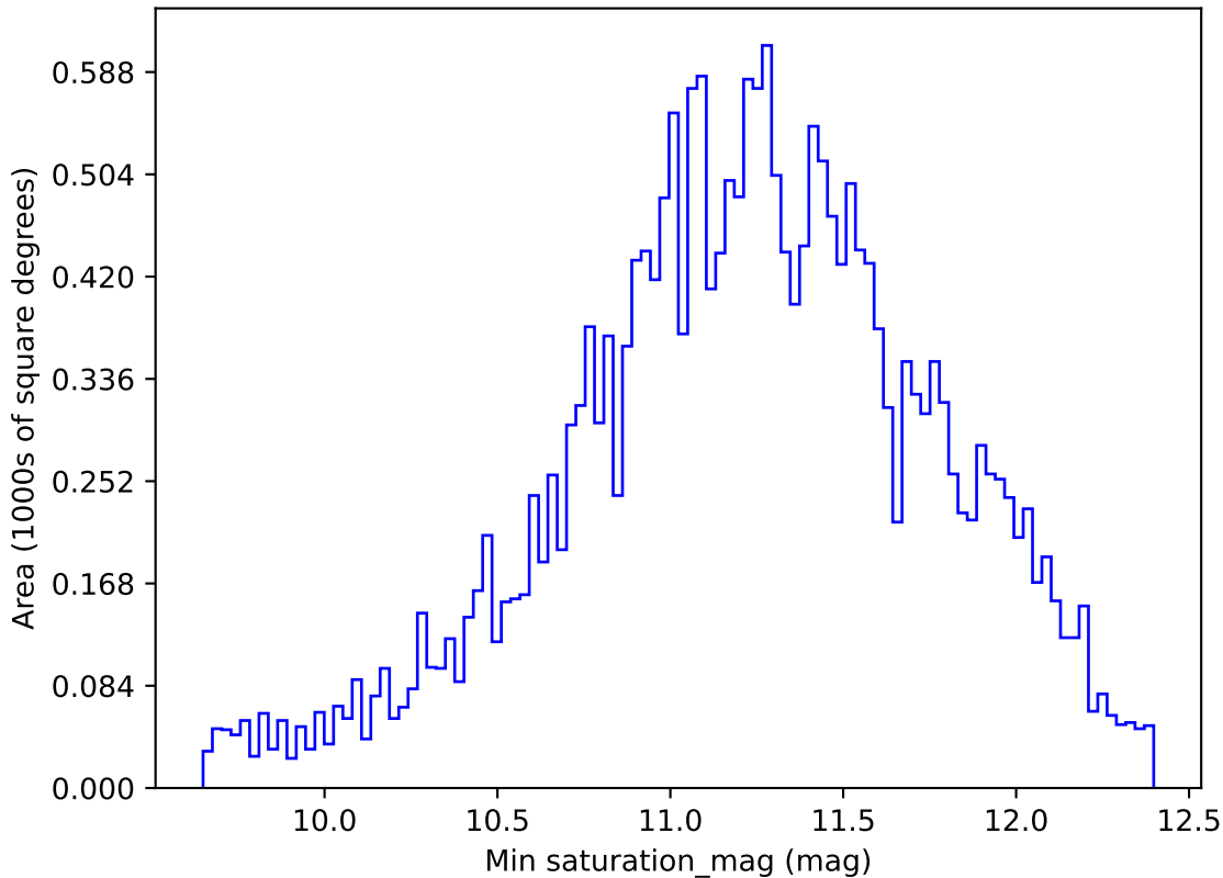
too_elab_r64_d2_giz_v3.4_10yrs All sky y band: Min saturation_mag
